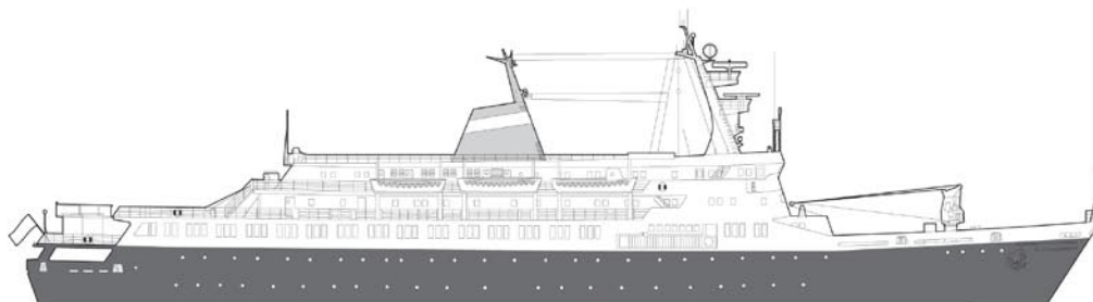
BRIDGE DECK CAPTAIN'S DECK UPPER DECK MAIN DECK LOWER DECK
